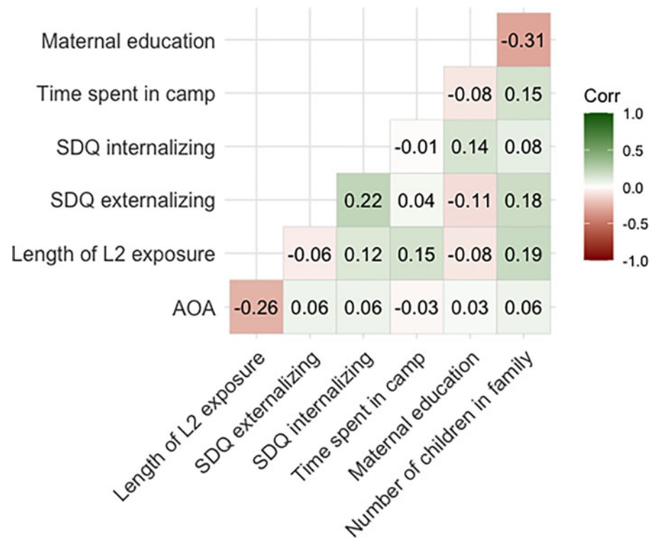
Figure 3. Correlation matrix for Individual difference predictors entered in regression models.
