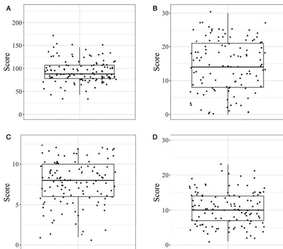
Figure 2. Boxplot of participant performance on the four tests, with the y-axis showing the possible range of scores for each test. Medians are indicated by the solid line. Note that the dispersion of the scores is partly a reflection of the scale of the task. For example, the range of vocabulary scores (2A) may appear deceptively small compared with scores from other tasks because the scale ranges from 0–228.
