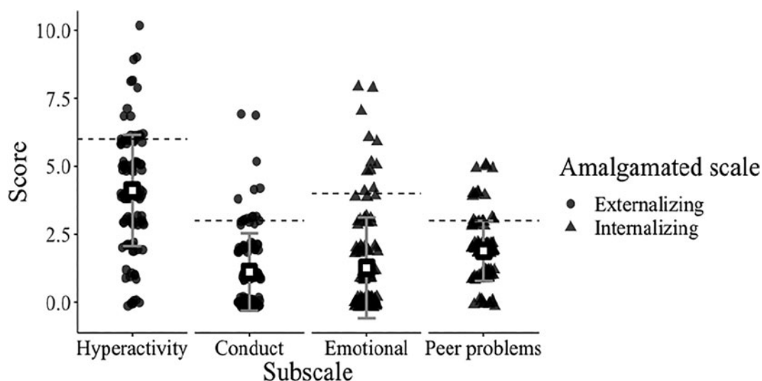
Figure 1. Participant scores according to SDQ subscale. Each circle and triangle denotes one participant. The white square indicates the mean for that subscale. The error bar indicates one SD below and above the mean. Horizontal, dashed, lines indicate borderline scores, which separate normal (lower) and abnormal (higher) scores. Shape indicates whether each subscale pertains to the externalizing (circle) or internalizing (triangle) amalgamated scales.
