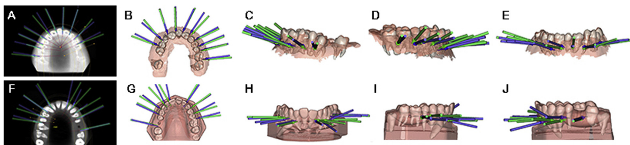
Fig 2. Deviations measurement procedure between planned ( green ) and performed ( blue ) orthodontic self-drilling ( A-E ) and orthodontic self-tapping microscrews study groups ( F-J ).
