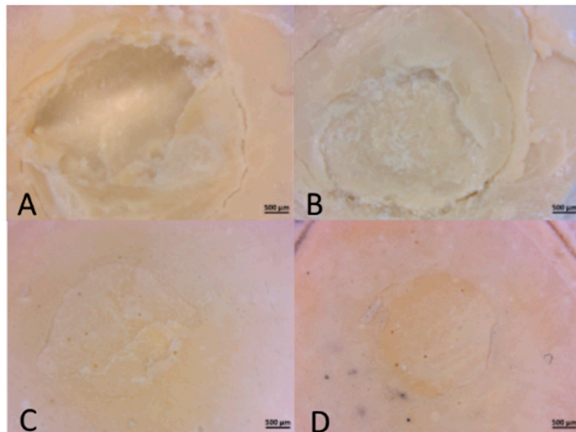
Figure 2. Stereomicroscopic images of the failure mode in different experimental groups under 0.945× magnification (scale bar = 500 μm). (A) Cohesive failure at 12 min in Biodentine self-etch; (B) cohesive failure at 12 min in Biodentine total etch (two steps); (C) adhesive failure at 24 h in Biodentine self-etch; (D) adhesive failure at 24 h in Biodentine total etch (two steps).
